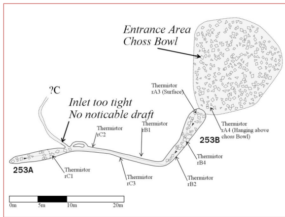
Fig. 2: Survey of Rundreishöhle (1623/253), annotated with sensor placements for data collection. 253a and b are entrances, and ?C denotes an extremely tight passage which has not been explored. Arrows designate slope; they point downhill. Weather station was placed on the surface above 253b. North is up, see Fig. 3 for legend.
